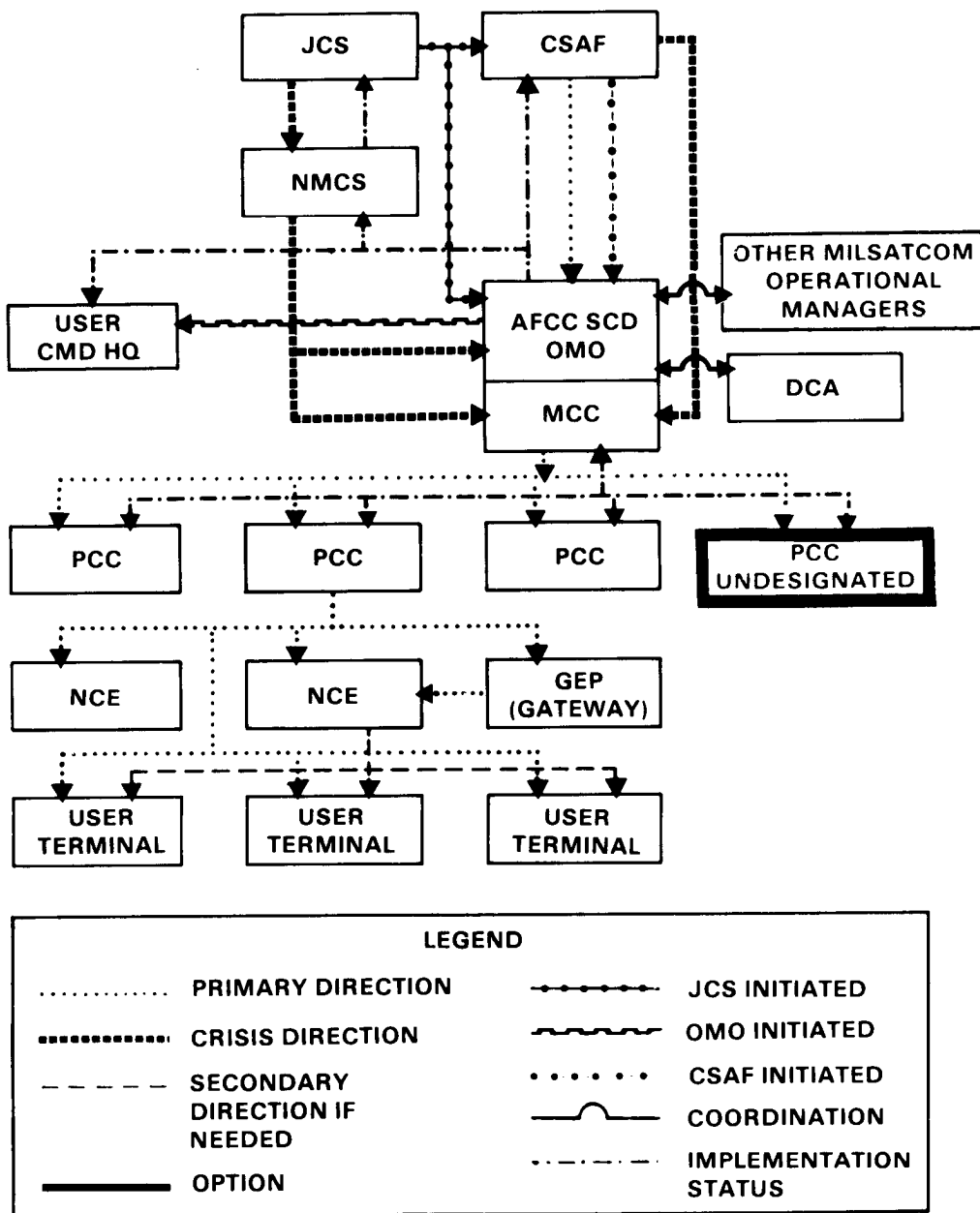
Figure 7-1. AFSATCOM system control hierarchy.
